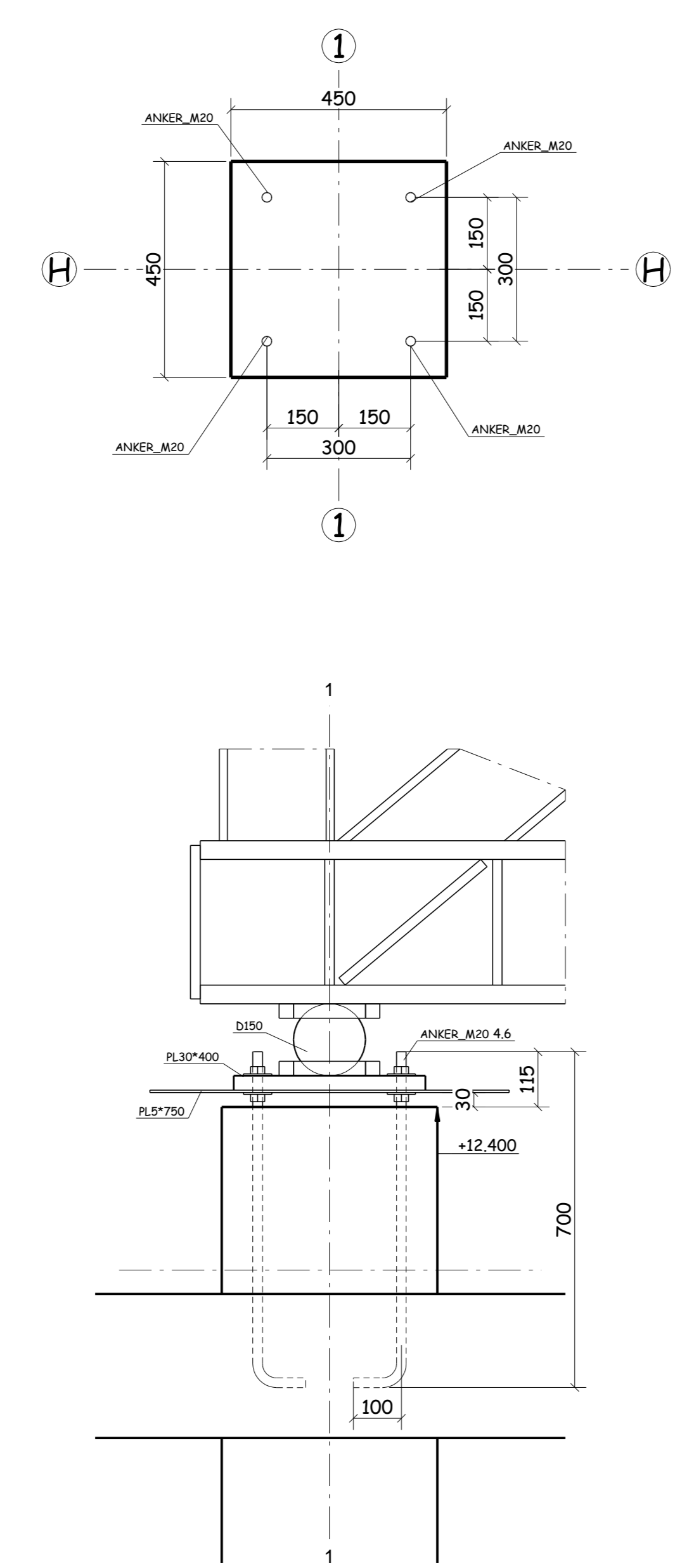
DETAIL ANKERS
