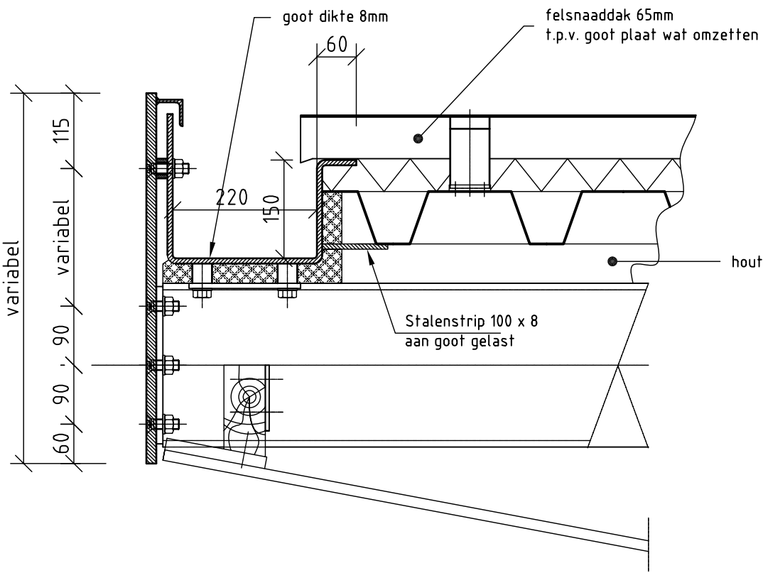
detail H
