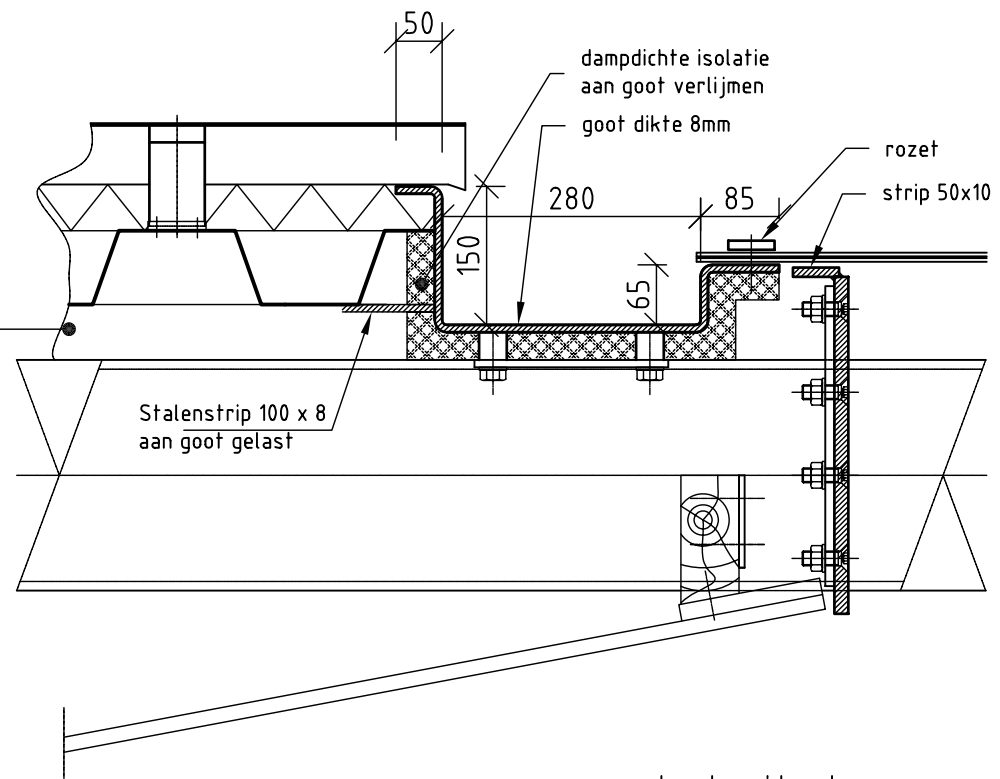
detail J
