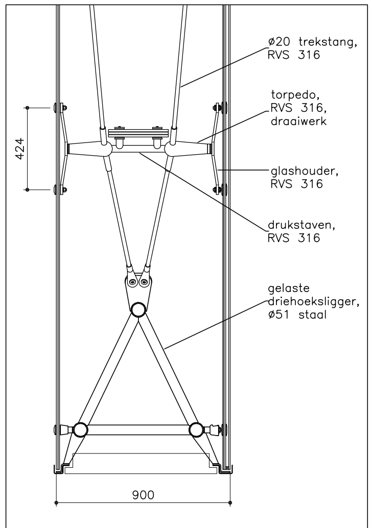
DETAIL SPANT
